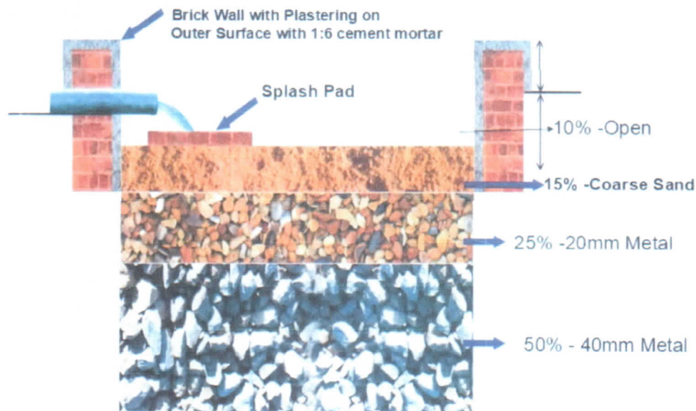
Rain water Harvester pit diagram
