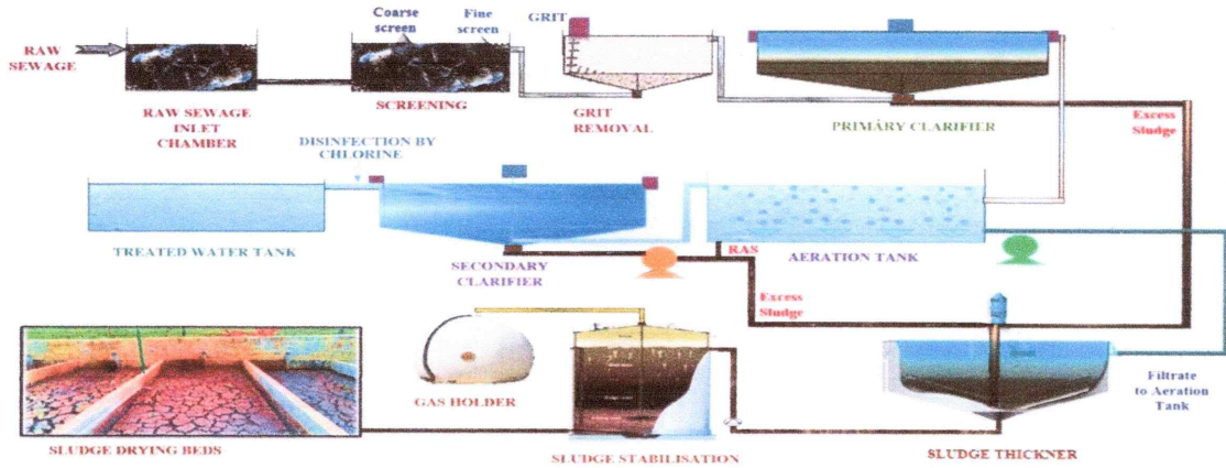
Sewage Treatment Process
