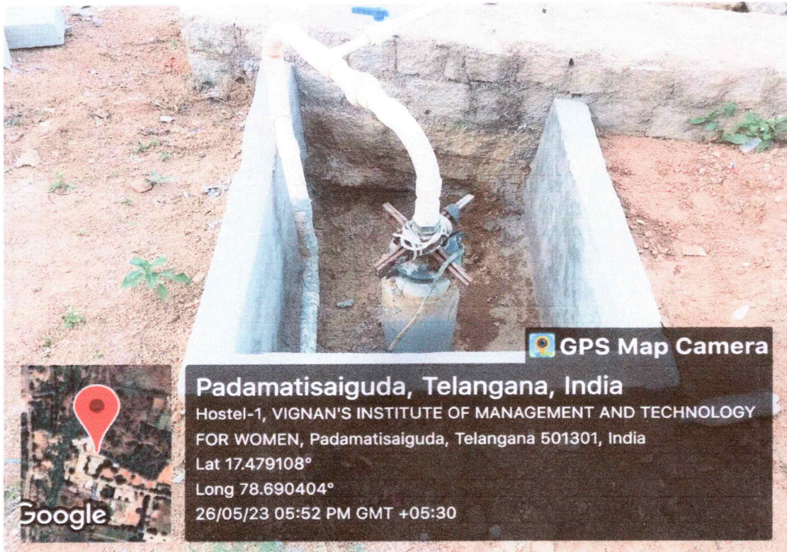
Bore well Recharge
