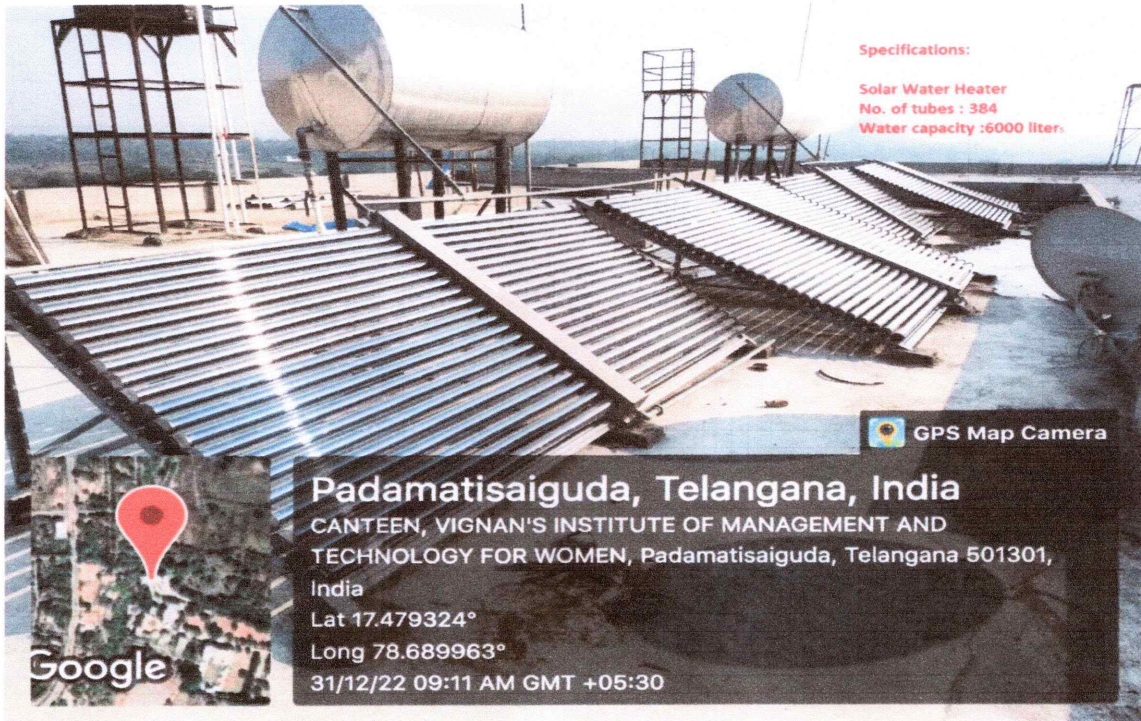
Solar water heater tubes producing 6000 liters of hot water
