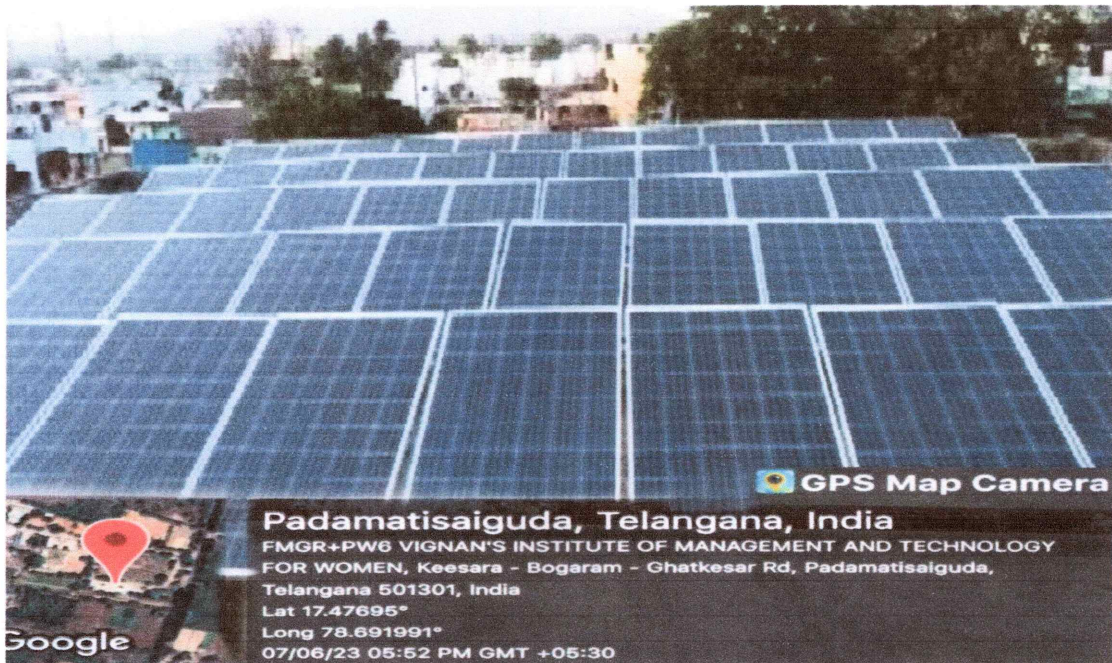
Solar Power Panel on the rooftop with a capacity of 50kW
